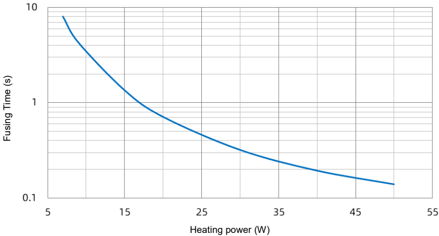
SHJ 15 A Power-Time Curve
